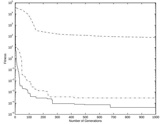
Fig. 4. Convergence procedures of CSA, SA, and hybrid algorithm in 50-dimension Zakharov function optimization. Dash-dotted line: CSA, dash line: SA method, solid line: hybrid algorithm.
