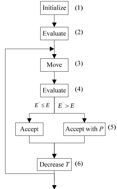
Fig. 2. Flow chart of basic SA method.
