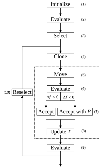
Fig. 3. Flow chart of hybrid optimization algorithm.
